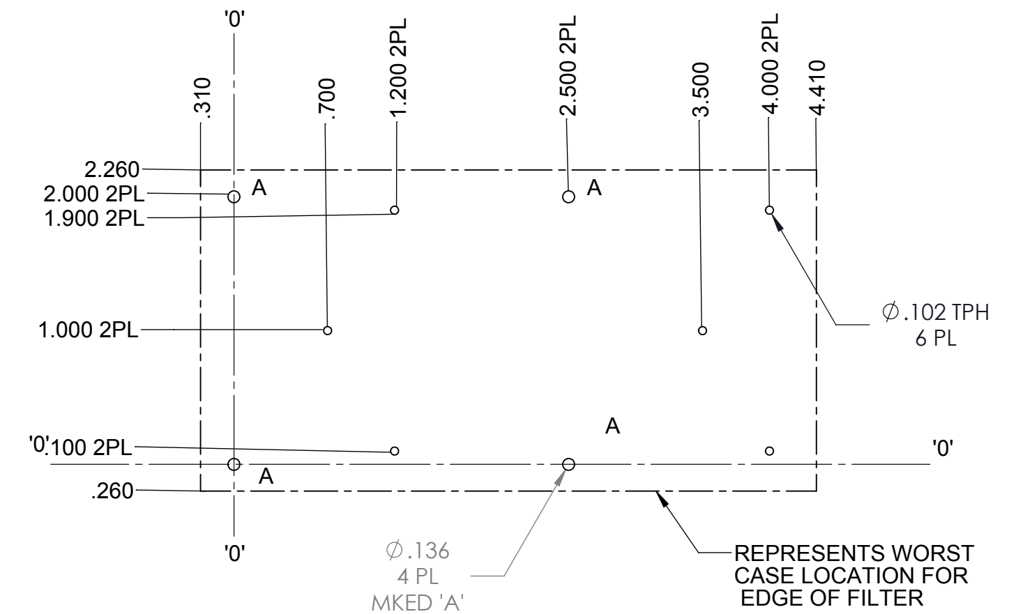
RECOMMENDED CUSTOMER MOUNTING (TOP VIEW)
