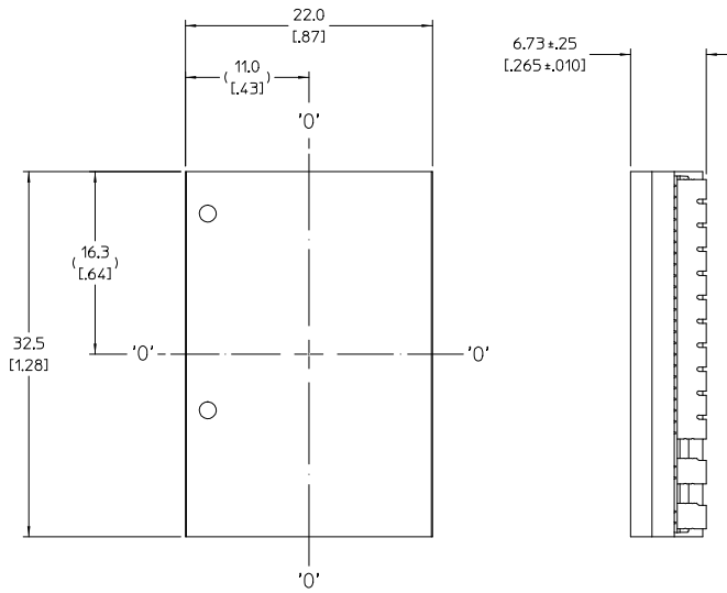
TOP VIEW (COMPONENT SIDE)
