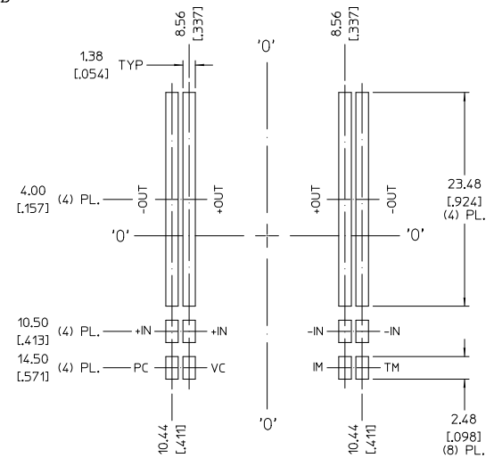
RECOMMENDED LAND PATTERN (COMPONENT SIDE SHOWN)
