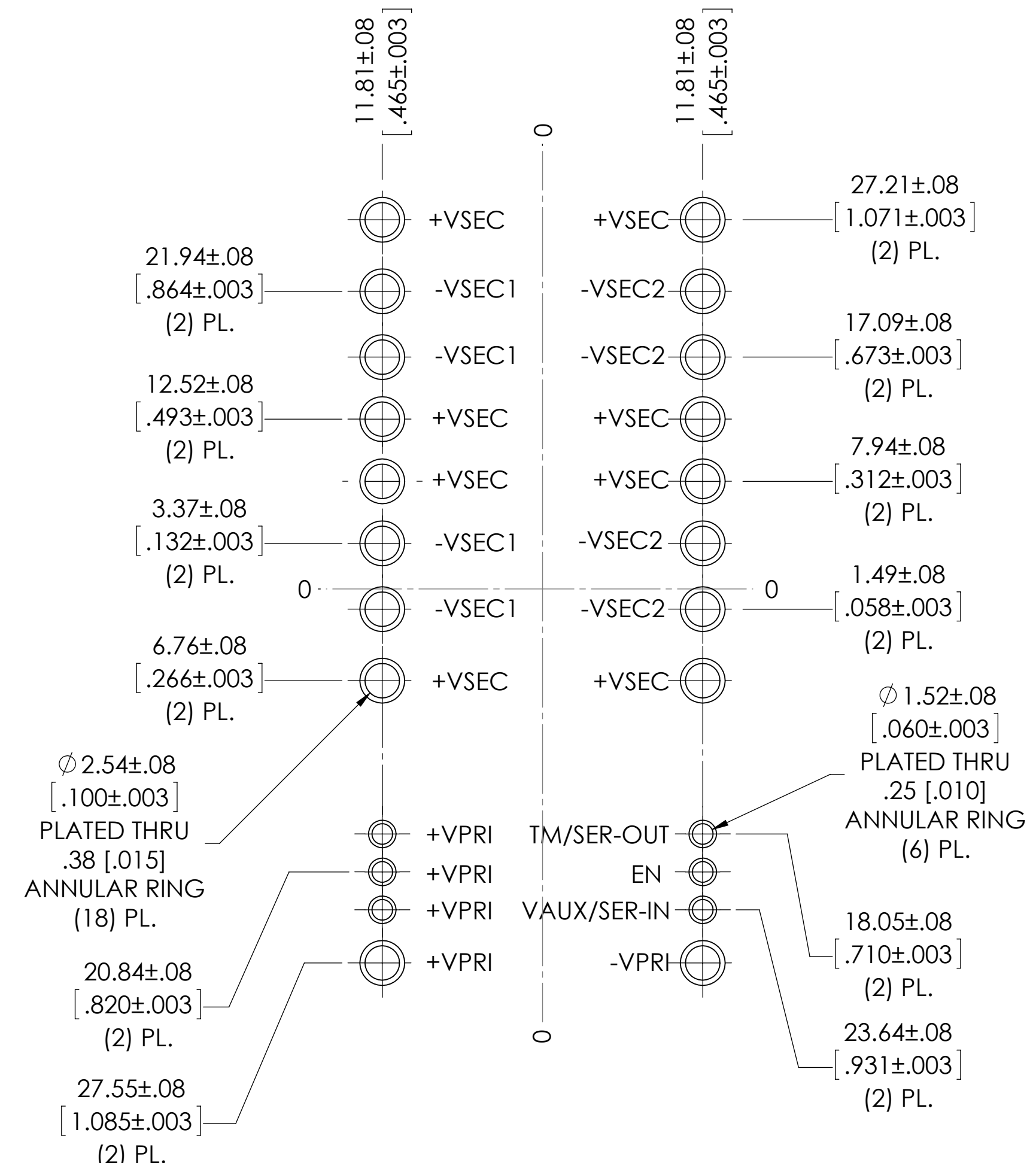
RECOMMENDED HOLE PATTERN (COMPONENT SIDE)
