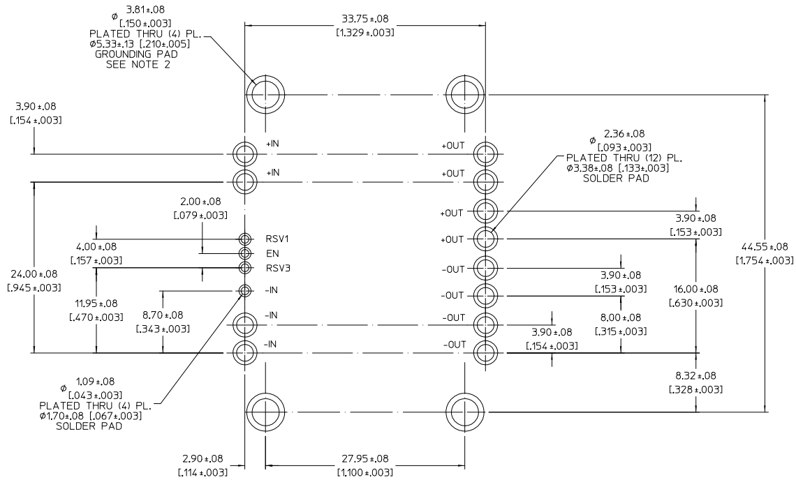
RECOMMENDED PCB PATTERN (COMPONENT SIDE SHOWN)
