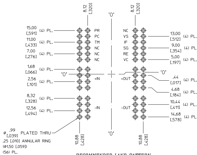
RECOMMENDED LAND PATTERN (COMPONENT SIDE SHOWN)
