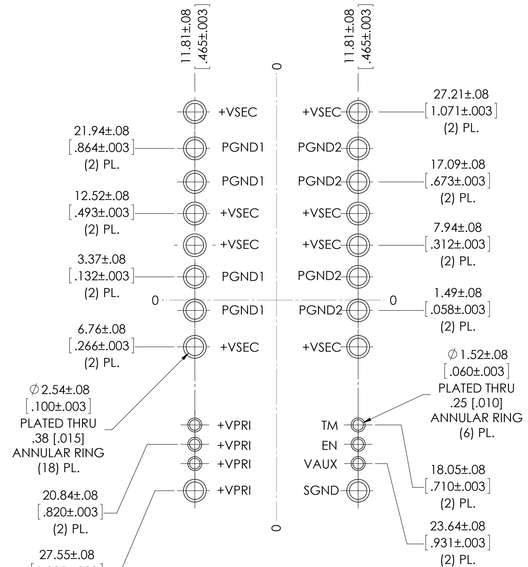
RECOMMENDED HOLE PATTERN (COMPONENT SIDE)
